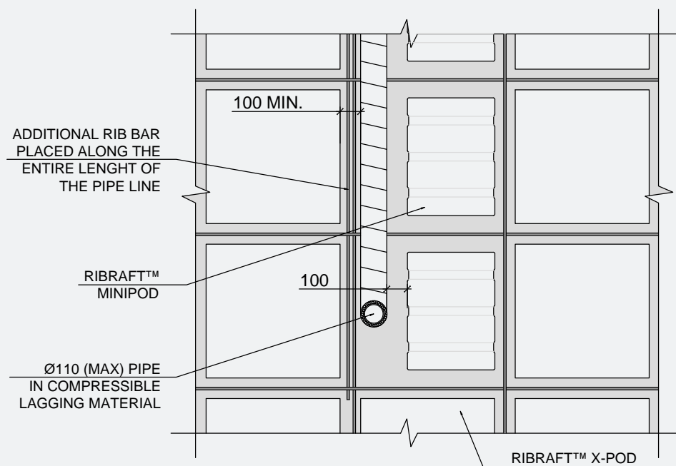
FIGURE 13: Use of X-Pod® Mini Pods to create zone for pipes to run without compromising Ribs
