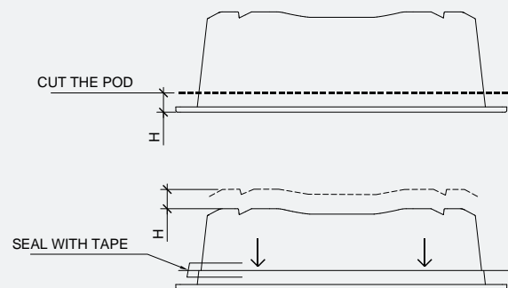
FIGURE 18: How to adjust depth of pod (cut) to suit rebate
