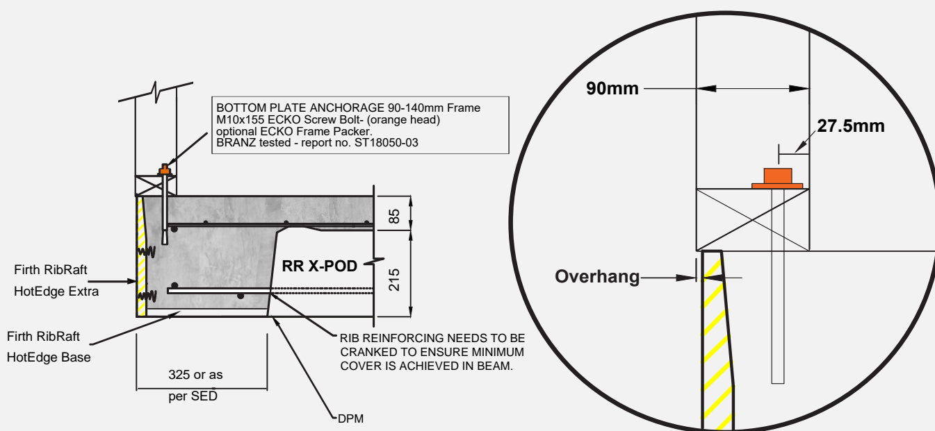
FIGURE 19: OVERHANG DETAIL FOR 90MM FRAMING WITH HOTEDGE EXTRA
