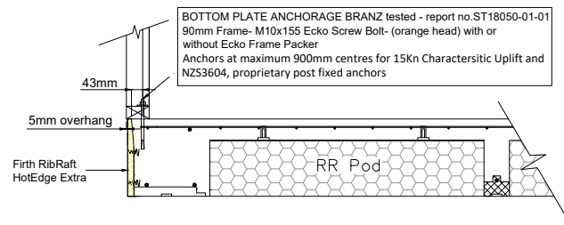
① 220mm FIRTH RIBRAFT POLYPOD 90mm WALL FRAME HOTEDGE EXTRA FIRTH RAFTMIX 20 OR 25MPa
