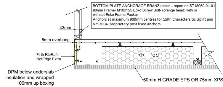
③ 220mm FIRTH RIBRAFT POLYPOD 90mm WALL FRAME HOTEDGE EXTRA & UNDERSLAB INSULATION FIRTH RAFTMIX 20 OR 25MPa
