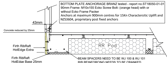
② 220mm FIRTH RIBRAFT POLYPOD 90mm WALL FRAME HOTEDGE EXTRA & HOTEDGE BASE FIRTH RAFTMIX 20 OR 25MPa
