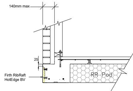
⑨ 220mm FIRTH RIBRAFT POLYPOD BRICK VENEER HOTEDGE FIRTH RAFTMIX 20 OR 25MPa
