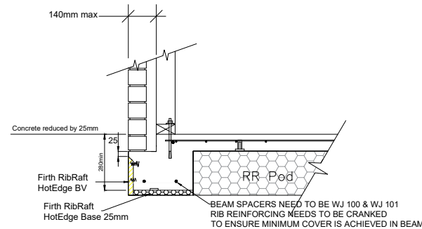
⑩ 220mm FIRTH RIBRAFT POLYPOD BRICK VENEER HOTEDGE & HOTEDGE BASE FIRTH RAFTMIX 20 OR 25MPa
