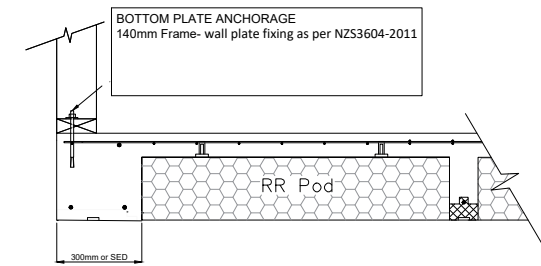
⑧ 220mm FIRTH RIBRAFT POLYPOD 90mm WALL FRAME FIRTH RAFTMIX 20 OR 25MPa
