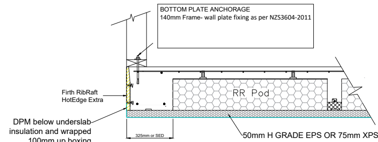
⑦ 220mm FIRTH RIBRAFT POLYPOD 140mm WALL FRAME HOTEDGE EXTRA & UNDERSLAB INSULATION FIRTH RAFTMIX 20 OR 25MPa
