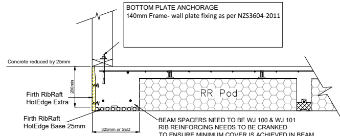
⑥ 220mm FIRTH RIBRAFT POLYPOD 140mm WALL FRAME HOTEDGE EXTRA & HOTEDGE BASE FIRTH RAFTMIX 20 OR 25MPa
