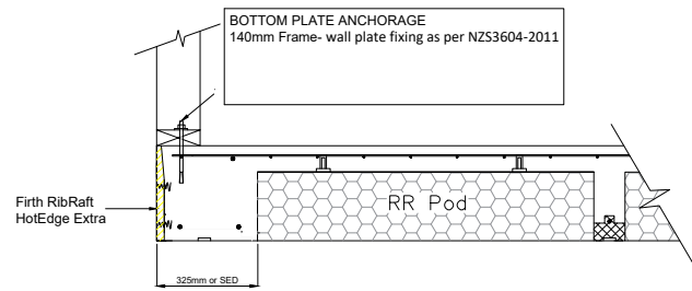
⑤ 220mm FIRTH RIBRAFT POLYPOD 140mm WALL FRAME HOTEDGE EXTRA FIRTH RAFTMIX 20 OR 25MPa
