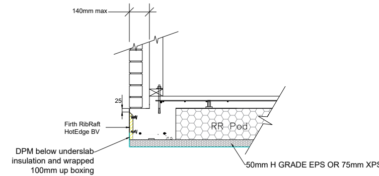
⑪ 220mm FIRTH RIBRAFT POLYPOD BRICK VENEER HOTEDGE & UNDERSLAB INSULATION FIRTH RAFTMIX 20 OR 25MPa
