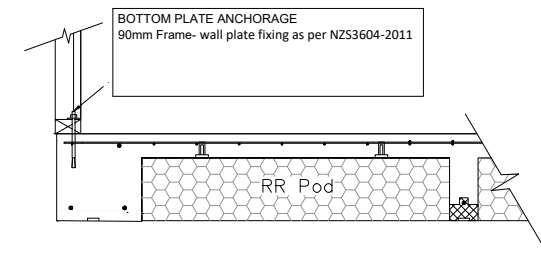
④ 220mm FIRTH RIBRAFT POLYPOD 90mm WALL FRAME FIRTH RAFTMIX 20 OR 25MPa
