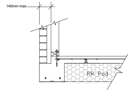
⑫ 220mm FIRTH RIBRAFT POLYPOD BRICK VENEER FIRTH RAFTMIX 20 OR 25MPa
