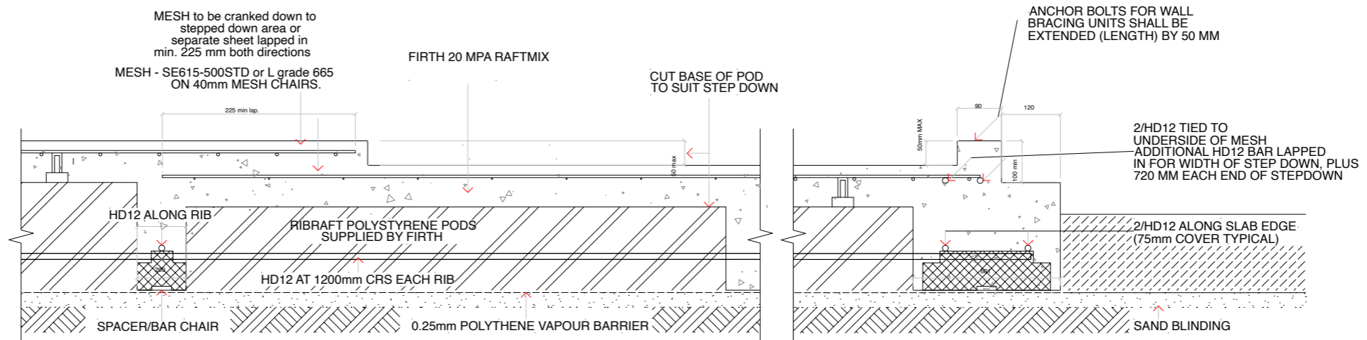
RIB RAFT FLOOR - SET-DOWN DETAIL FOR MAX. 50mm REBATED SHOWER
